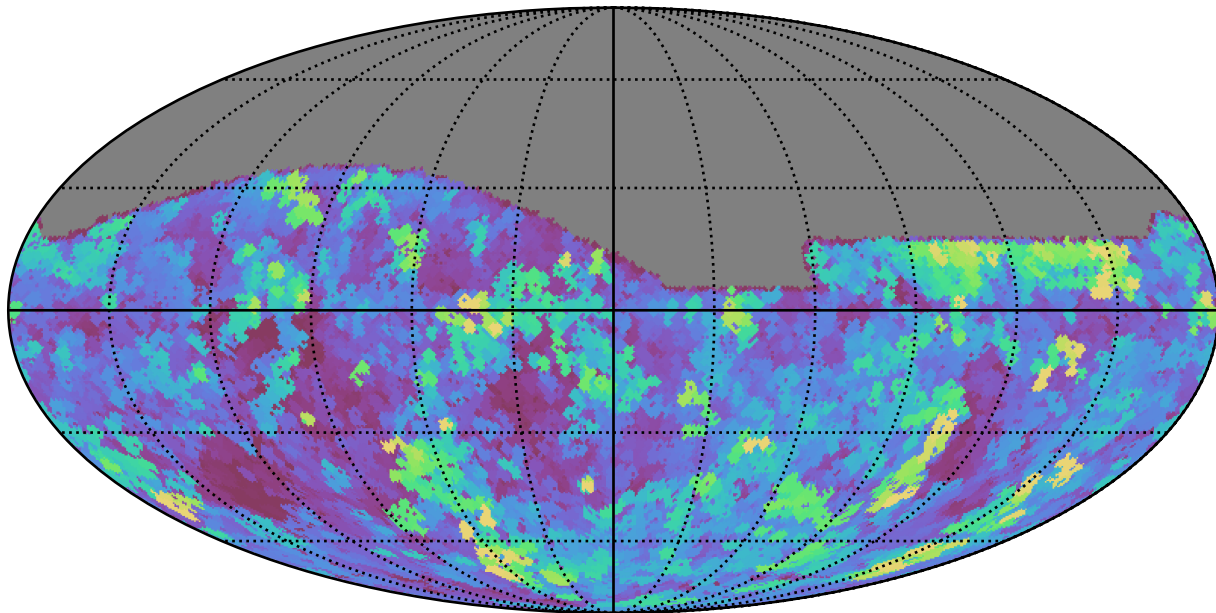
too_combined_s1.0_v3.4_10yrs All sky g band: Max seeingEff
