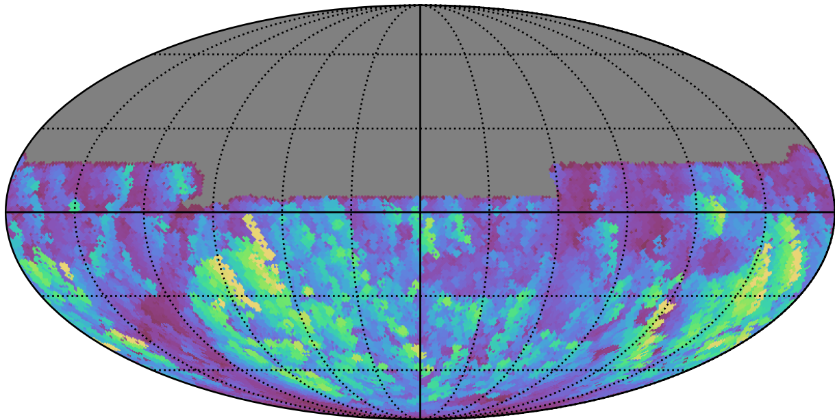
too_combined_s1.0_v3.4_10yrs All sky u band: Max normairmass
