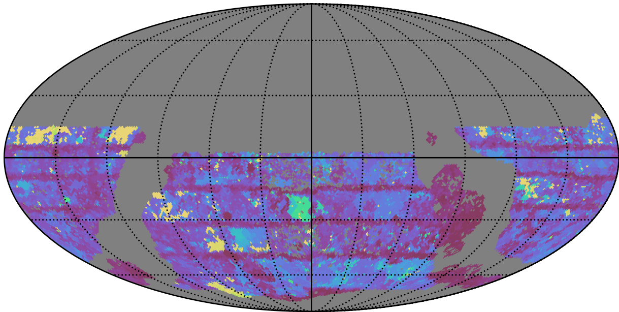
too_combined_s1.0_v3.4_10yrs WFD i band: Max Inter-Night Gap
