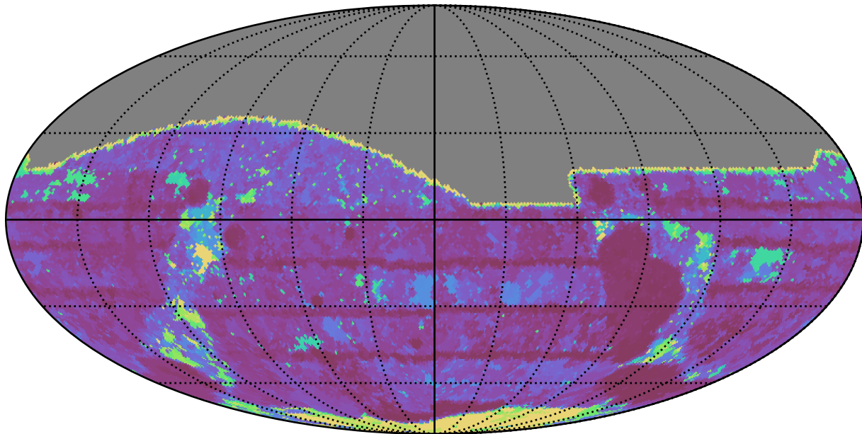
too_combined_s1.0_v3.4_10yrs All sky r band: Max Inter-Night Gap
