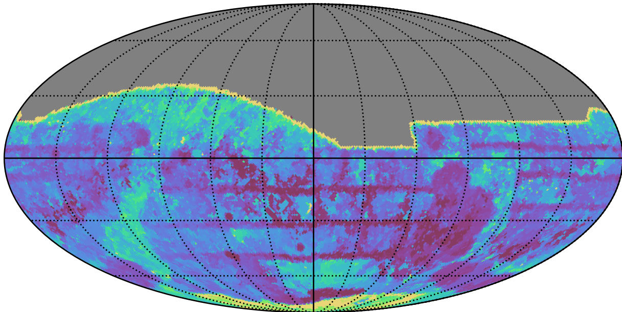
too_combined_s1.0_v3.4_10yrs All sky all bands: Max Inter-Night Gap
