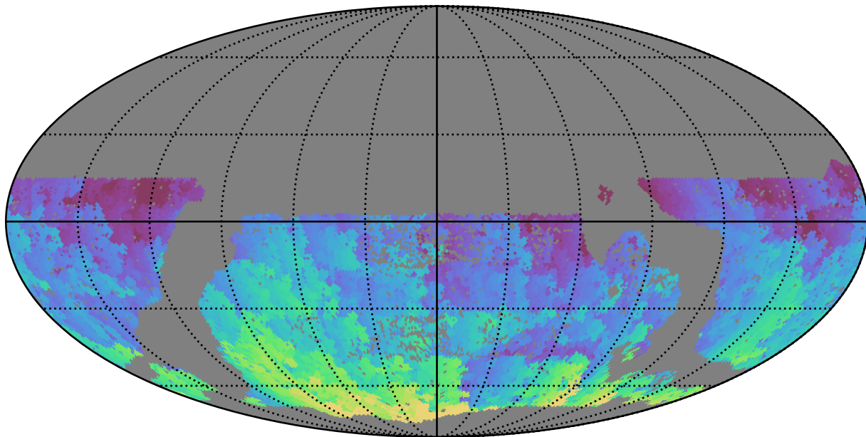
too_combined_s1.0_v3.4_10yrs WFD u band: Max HA
