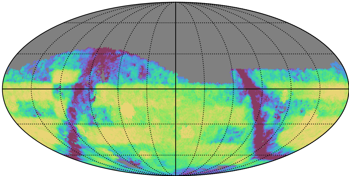
too_combined_s1.0_v3.4_10yrs Yr 3-4 i band: Exgal_CoaddM5
