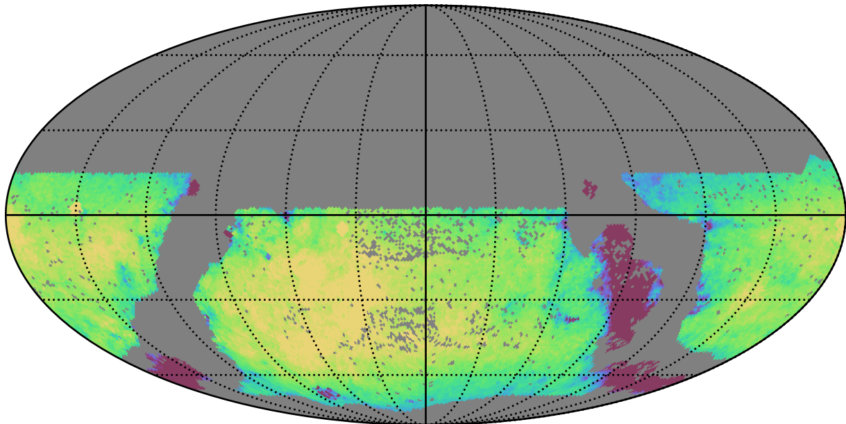
too_combined_s1.0_v3.4_10yrs WFD i band: Exgal_CoaddM5
