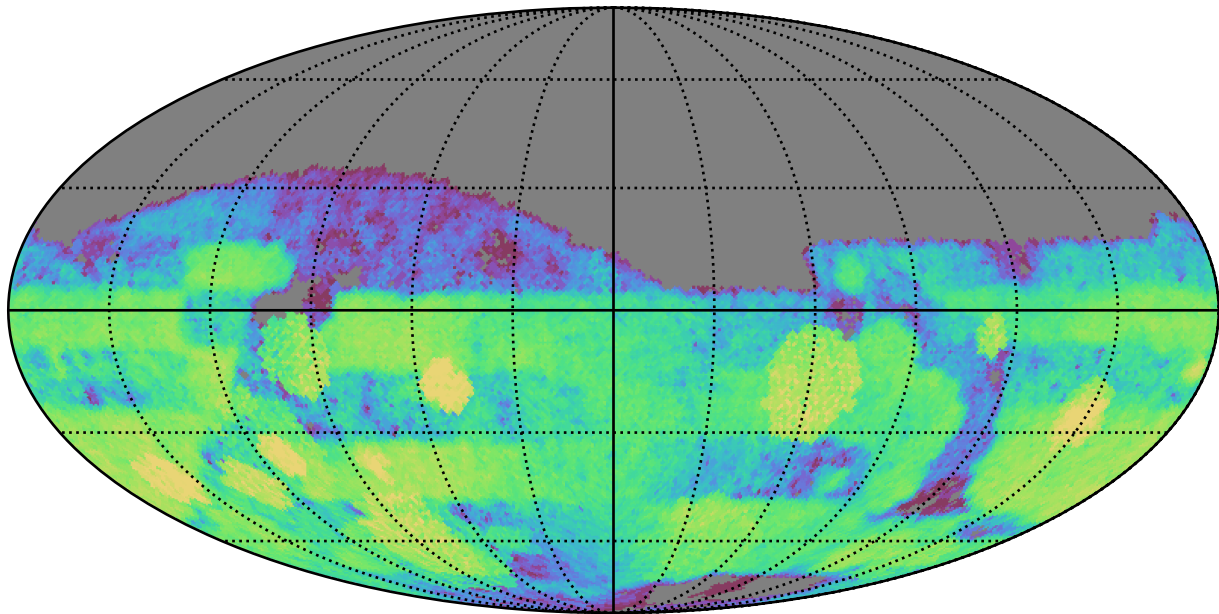
too_combined_s1.0_v3.4_10yrs Yr 3-4 r band: CoaddM5
