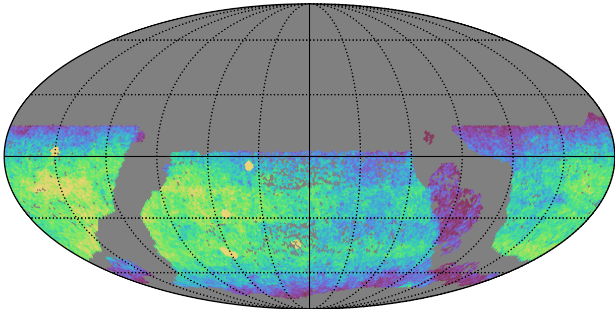
too_combined_s1.0_v3.4_10yrs WFD u band: CoaddM5
