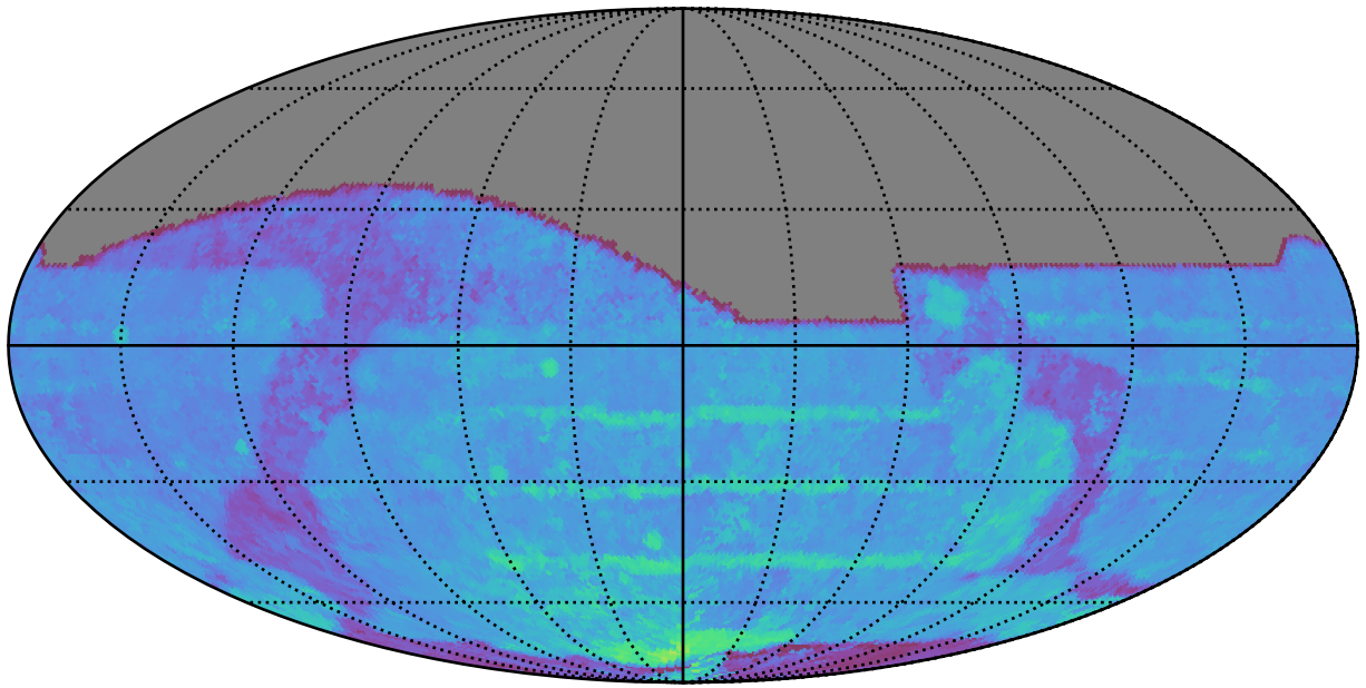
too_combined_s1.0_v3.4_10yrs All sky i band: 80thPercentile Season Length
