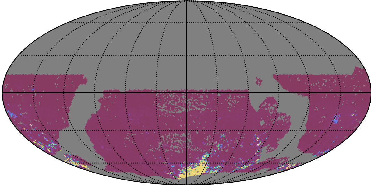
too_combined_s1.0_v3.4_10yrs WFD ri bands: 75th Percentile Intranight Timespan
