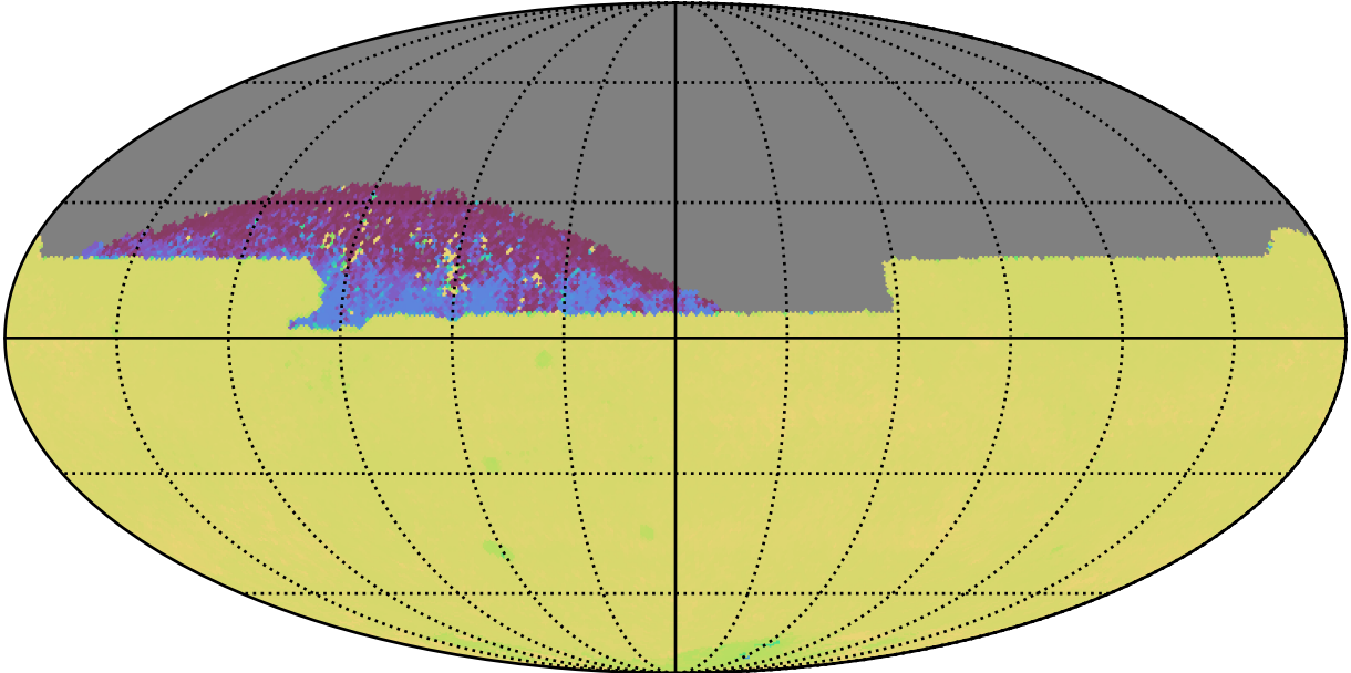
too_combined_s1.0_v3.4_10yrs All sky zy bands: 75th Percentile Intranight Timespan
