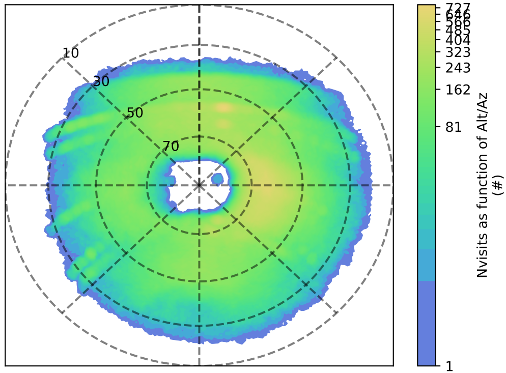
too_combined_s1.0_v3.4_10yrs u: Nvisits as function of Alt/Az
