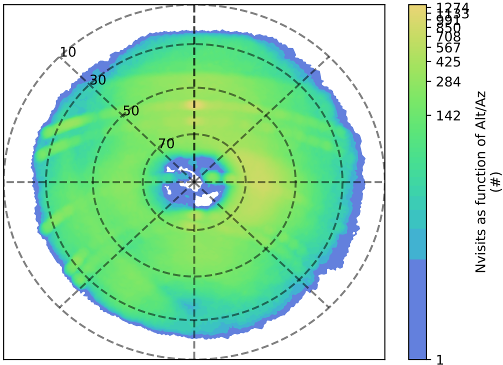
too_combined_s1.0_v3.4_10yrs g: Nvisits as function of Alt/Az
