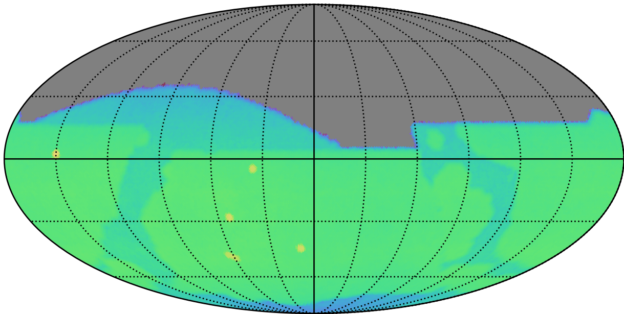
too_combined_s1.0_v3.4_10yrs r: CoaddM5
