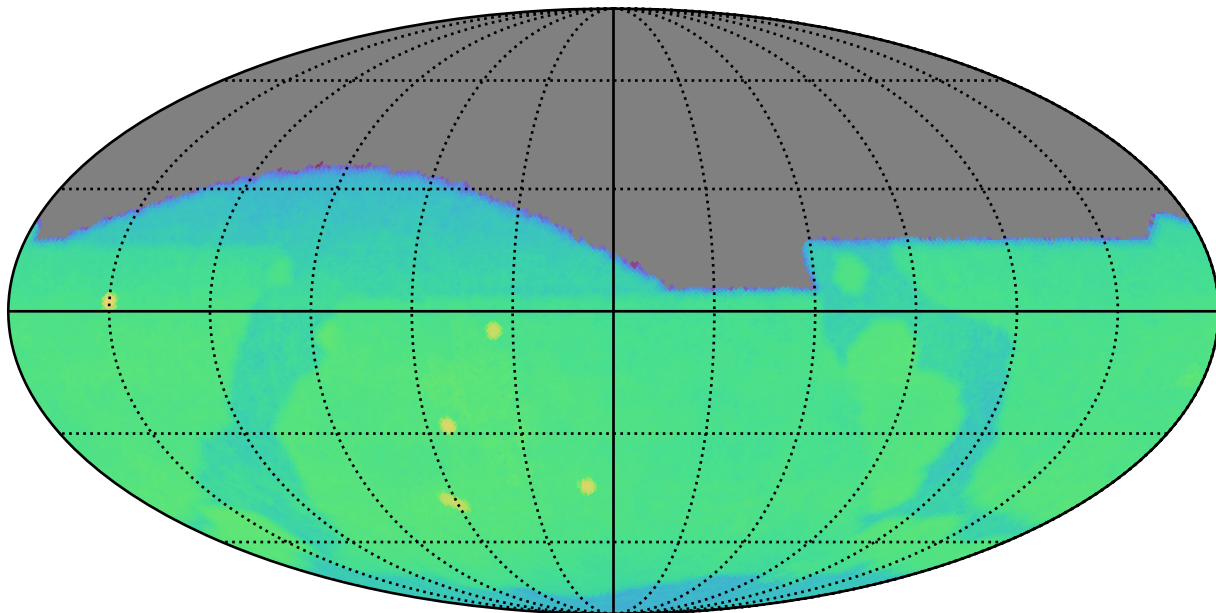
too_combined_s1.0_v3.4_10yrs g: CoaddM5
