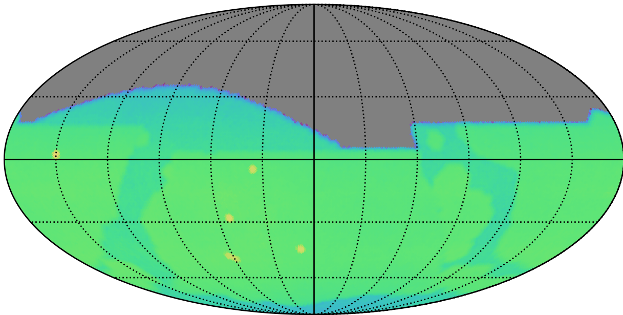
too_combined_s1.0_v3.4_10yrs : CoaddM5
