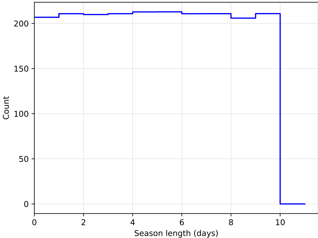
too_combined_s1.0_v3.4_10yrs DD:EDFS all bands: SeasonLength
