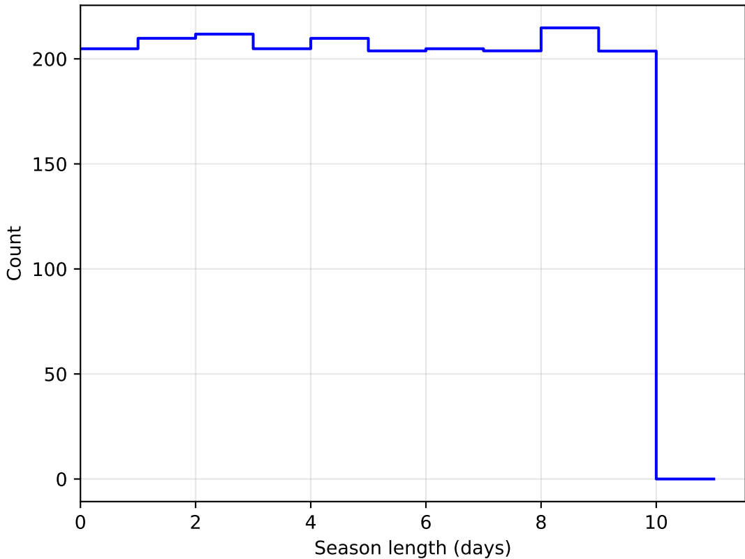
too_combined_s1.0_v3.4_10yrs DD:ECDFS all bands: SeasonLength
