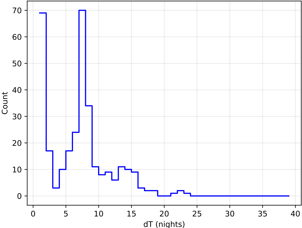
too_combined_s1.0_v3.4_10yrs all bands: DD:XMM_LSS Delta Nights Histogram
