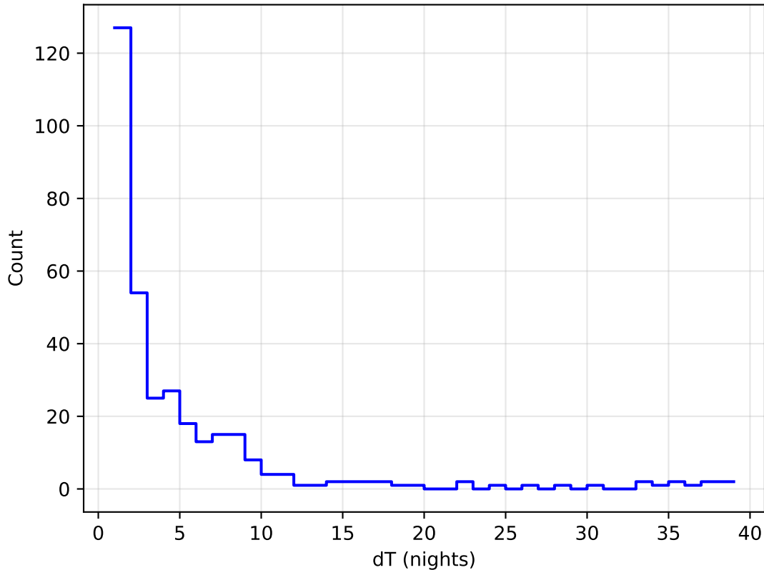
too_combined_s1.0_v3.4_10yrs all bands: DD:WFD Delta Nights Histogram
