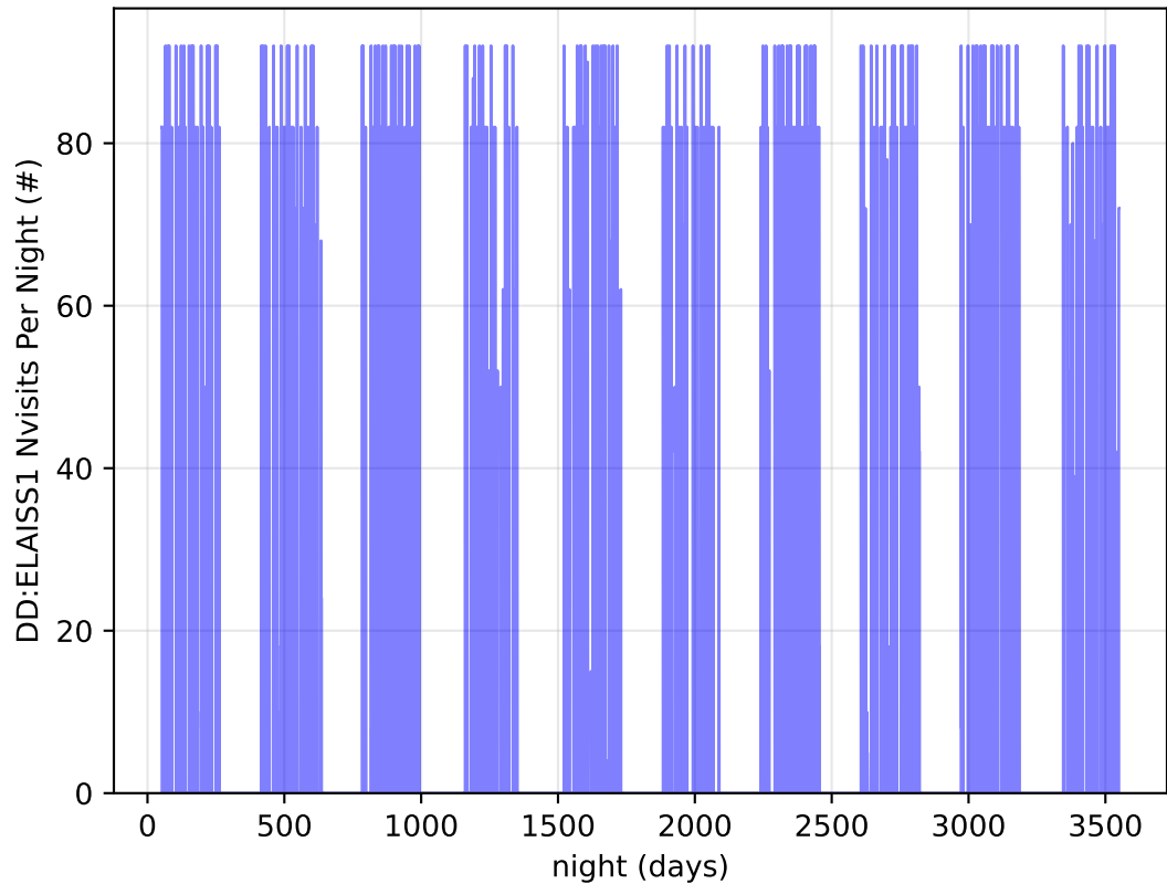
too_combined_s1.0_v3.4_10yrs all bands: DD:ELAISS1 Nvisits Per Night
