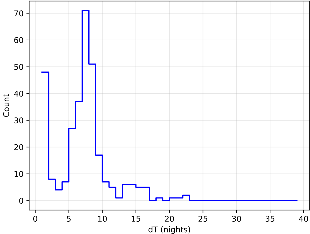
too_combined_s1.0_v3.4_10yrs all bands: DD:ELAISS1 Delta Nights Histogram
