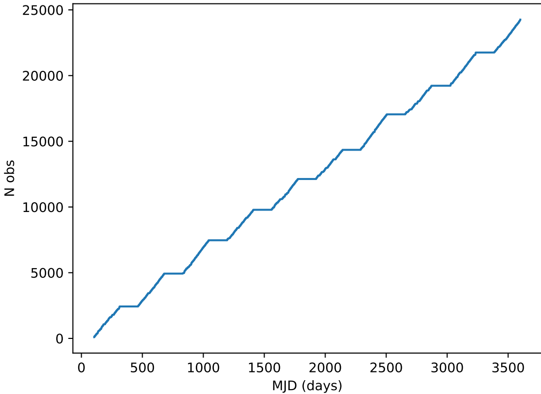
too_combined_s1.0_v3.4_10yrs all bands: DD:EDFS Cumulative NVisits
