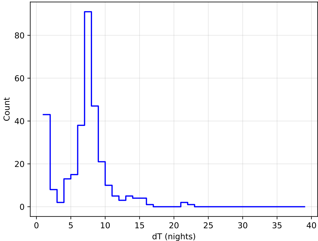
too_combined_s1.0_v3.4_10yrs all bands: DD:ECDFS Delta Nights Histogram
