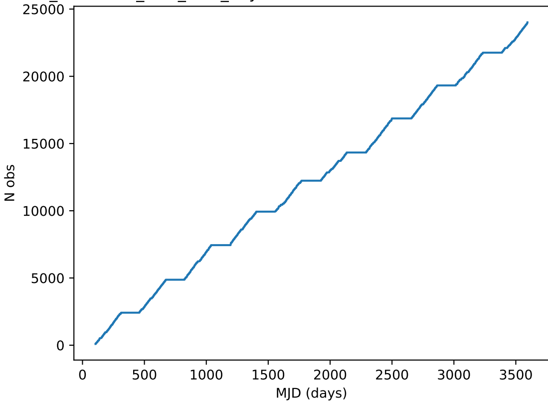
too_combined_s1.0_v3.4_10yrs all bands: DD:ECDFS Cumulative NVisits
