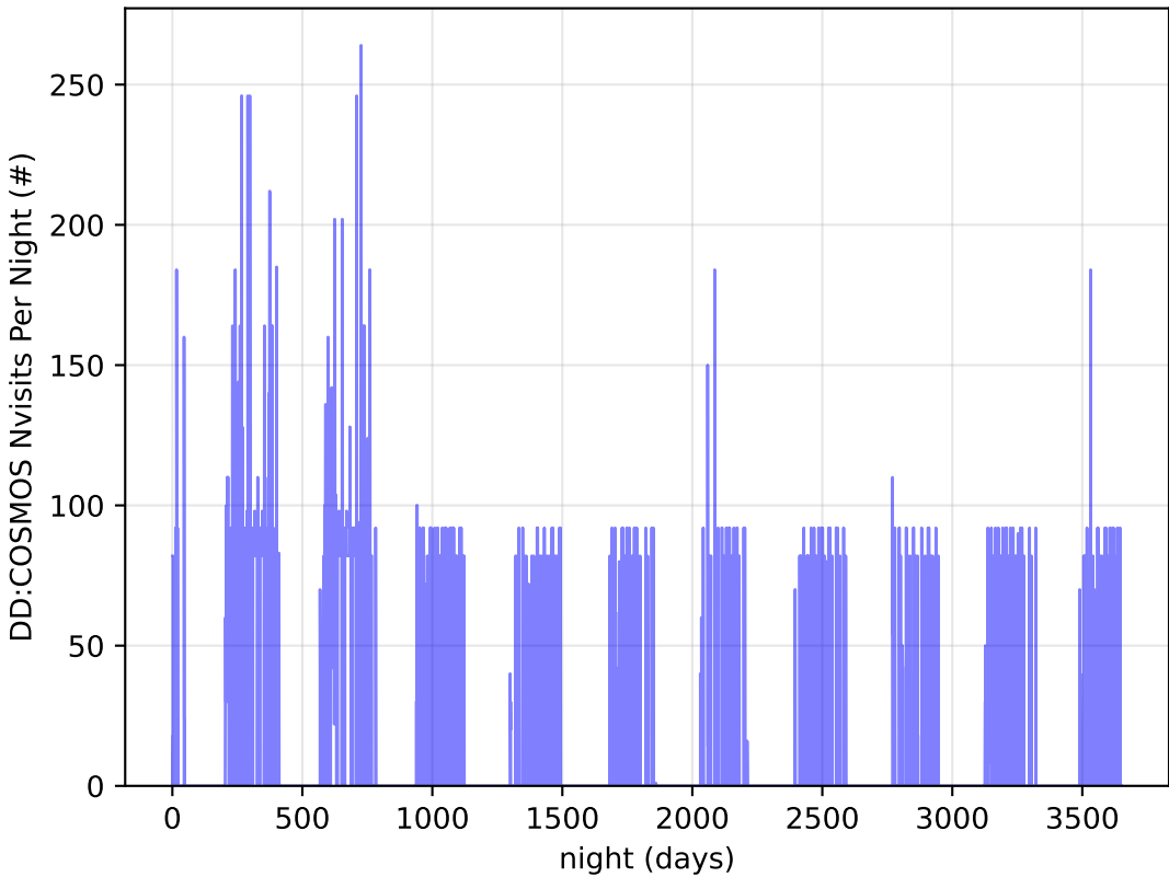
too_combined_s1.0_v3.4_10yrs all bands: DD:COSMOS Nvisits Per Night
