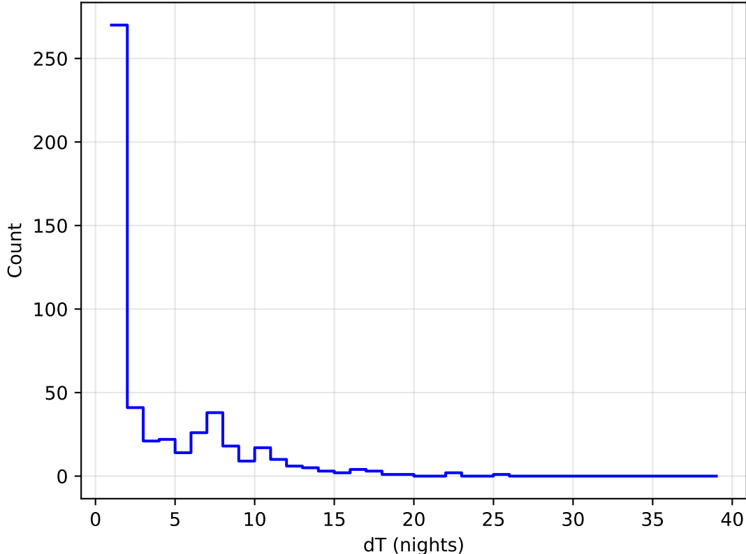
too_combined_s1.0_v3.4_10yrs all bands: DD: COSMOS Delta Nights Histogram
