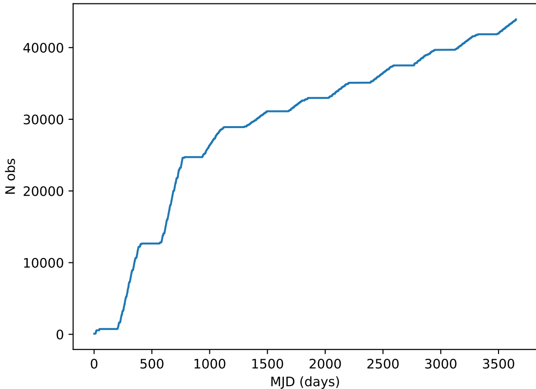
too_combined_s1.0_v3.4_10yrs all bands: DD: COSMOS Cumulative NVisits
