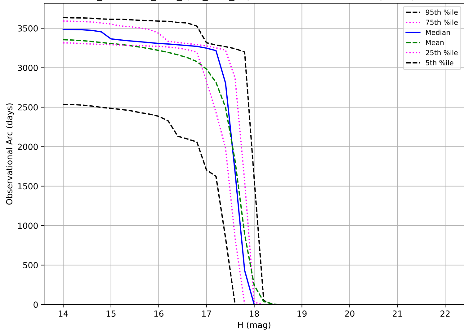
too_combined_s1.0_split_v3.4_10yrs: Observational Arc Length Trojan
