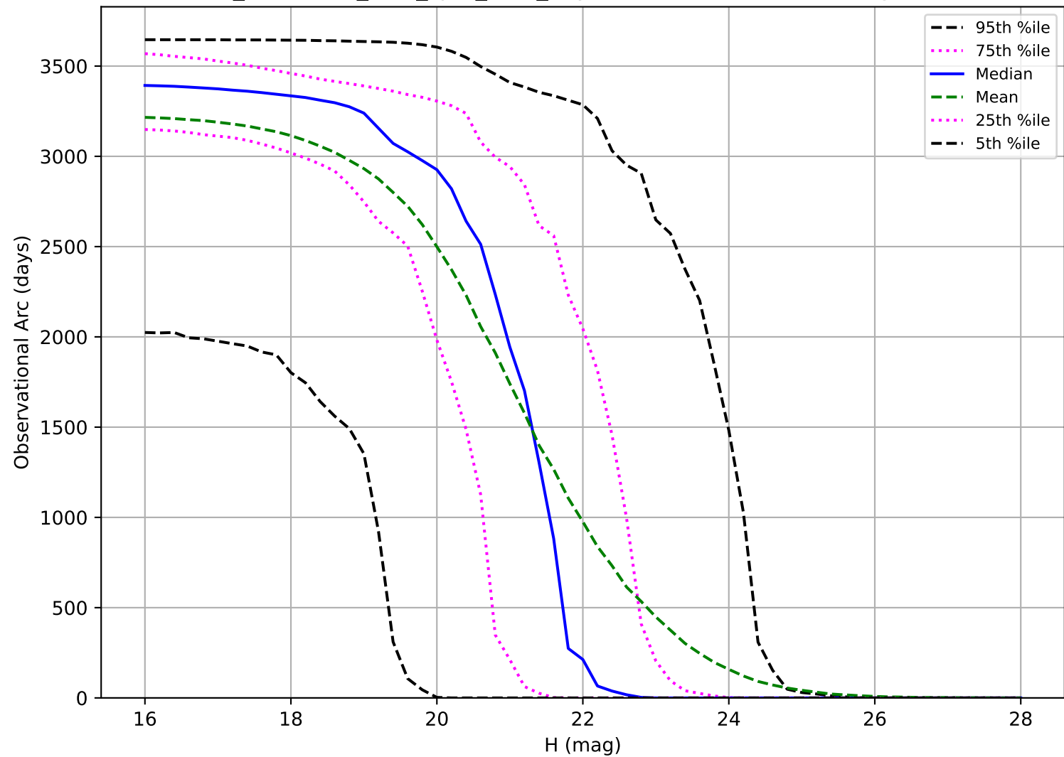
too_combined_s1.0_split_v3.4_10yrs: Observational Arc Length PHA
