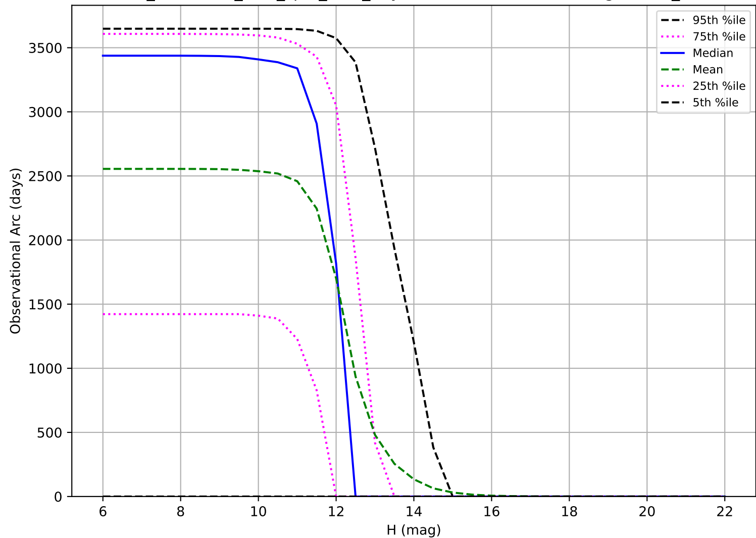
too_combined_s1.0_split_v3.4_10yrs: Observational Arc Length OCC_r20
