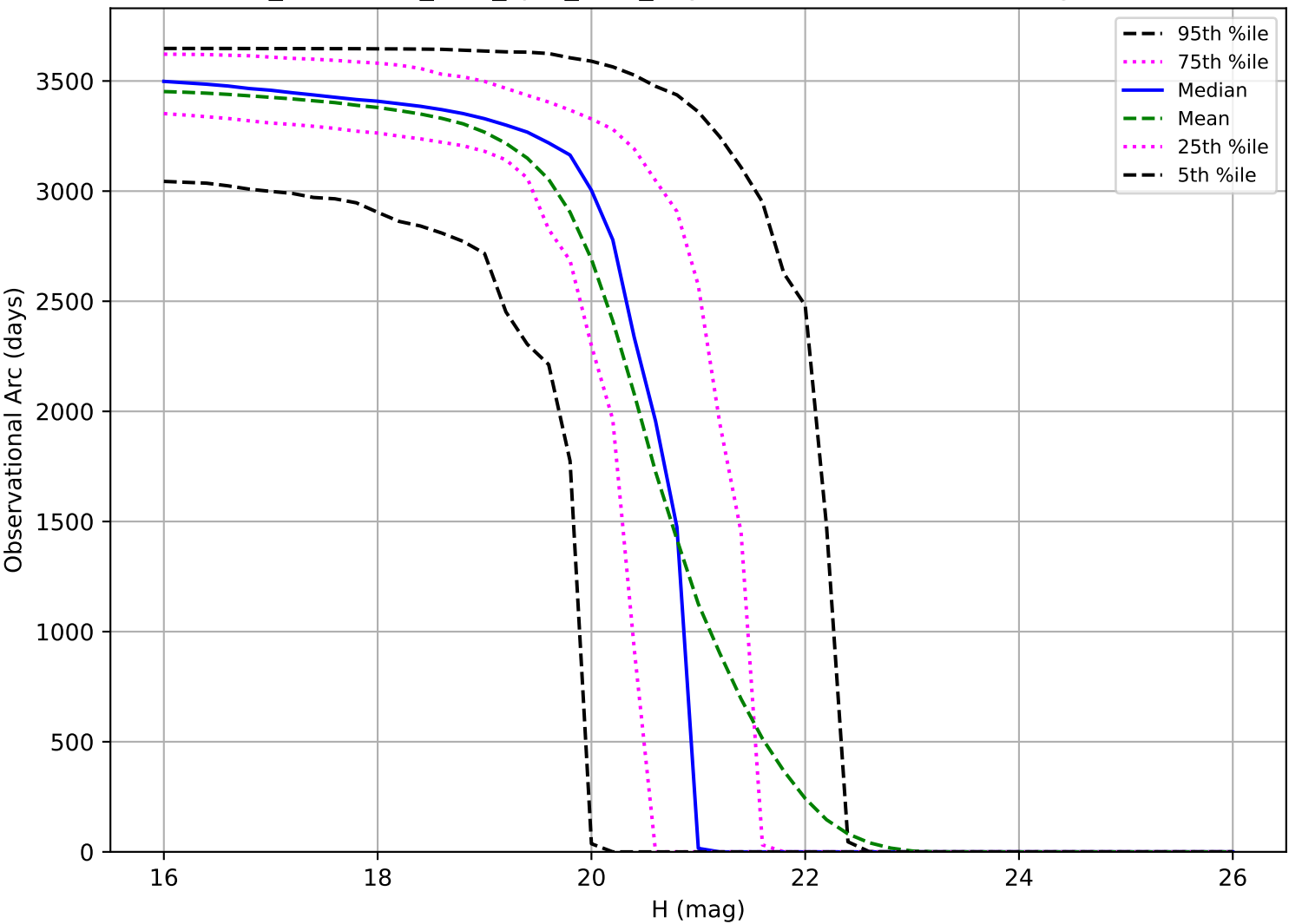
too_combined_s1.0_split_v3.4_10yrs: Observational Arc Length MBA
