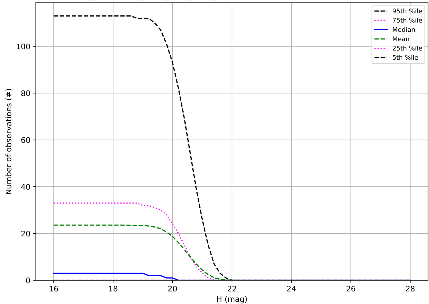
too_combined_s1.0_split_v3.4_10yrs: Number of observations Vatira
