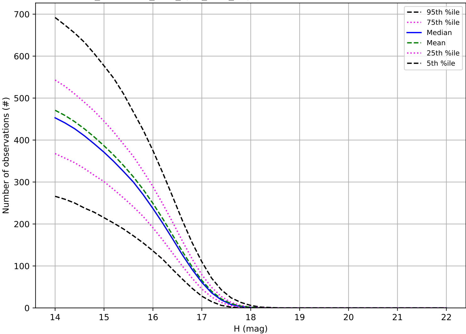
too_combined_s1.0_split_v3.4_10yrs: Number of observations Trojan
