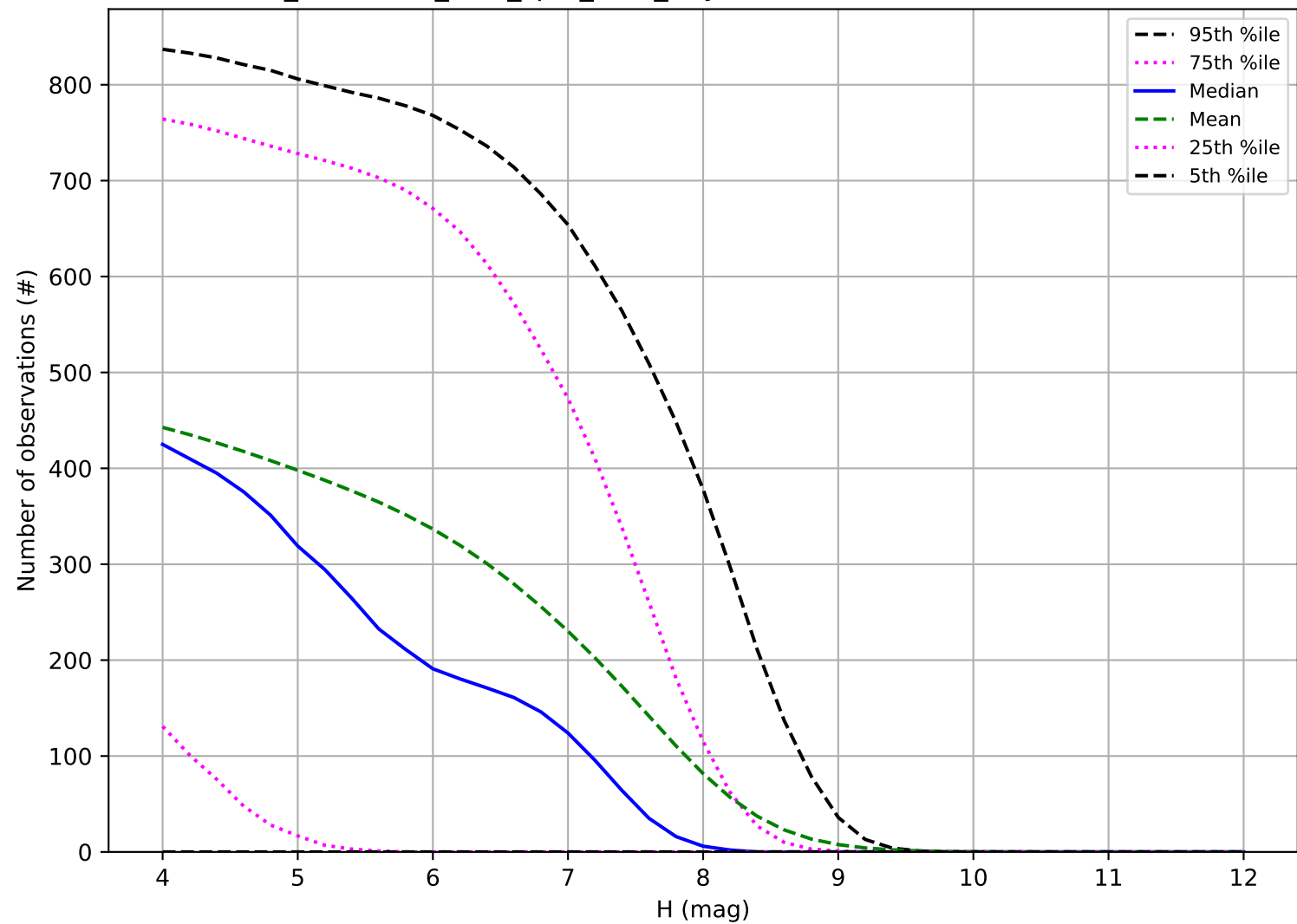
too_combined_s1.0_split_v3.4_10yrs: Number of observations TNO
