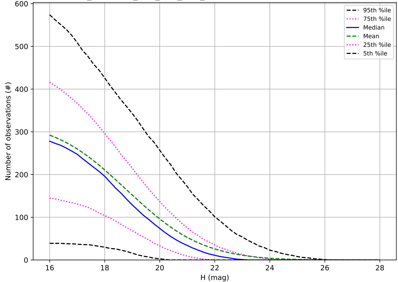
too_combined_s1.0_split_v3.4_10yrs: Number of observations PHA
