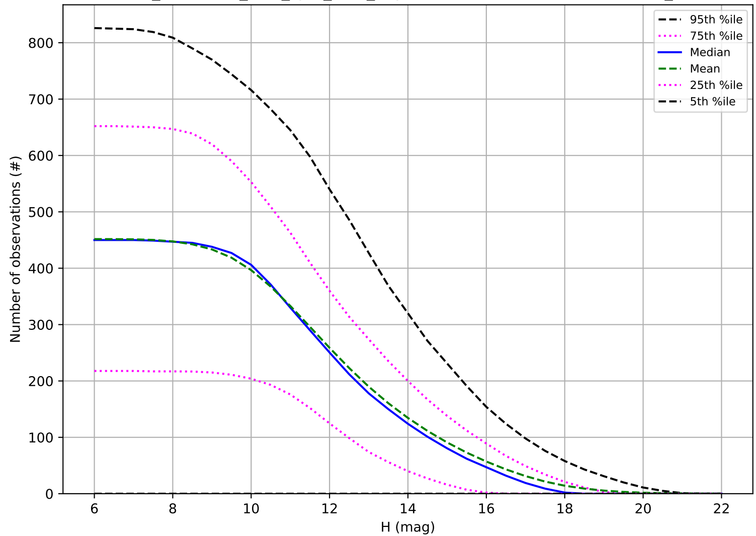
too_combined_s1.0_split_v3.4_10yrs: Number of observations OCC_r5
