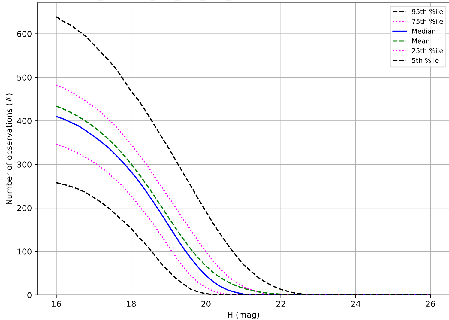
too_combined_s1.0_split_v3.4_10yrs: Number of observations MBA
