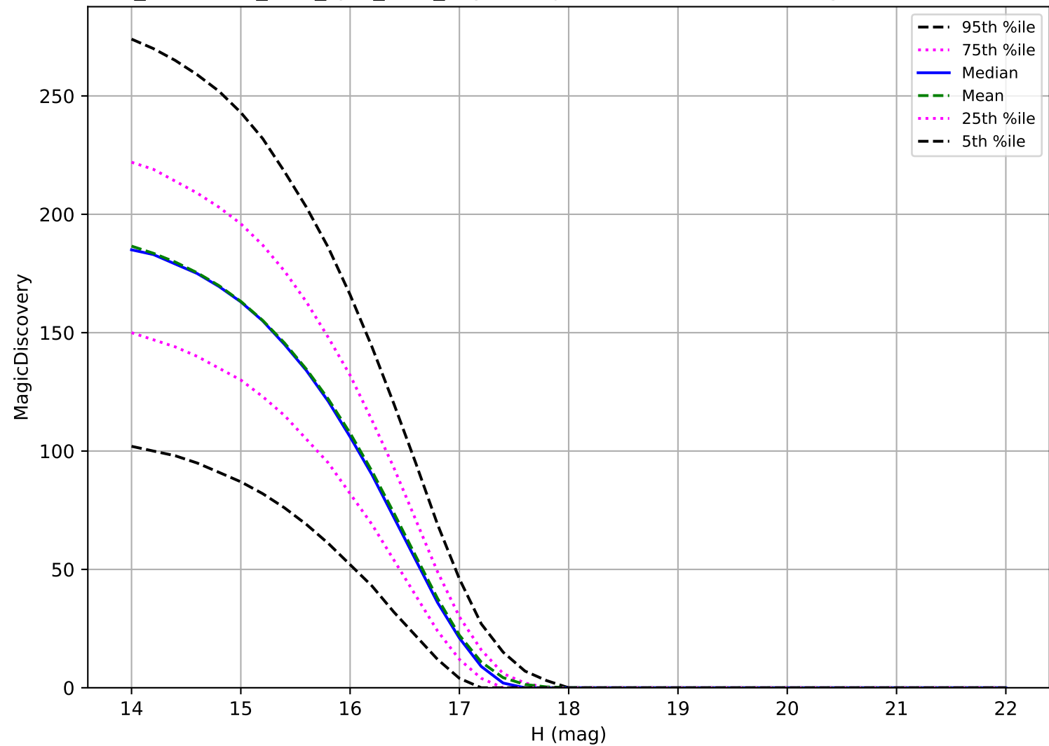
too_combined_s1.0_split_v3.4_10yrs: Trojan 6 detections in 60 nights detection loss
