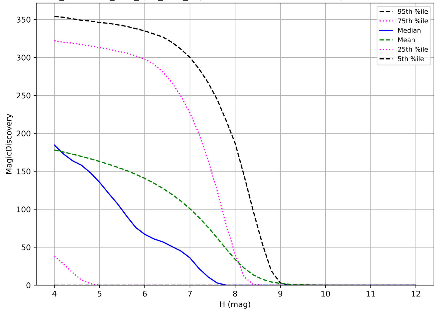
too_combined_s1.0_split_v3.4_10yrs: TNO 6 detections in 60 nights detection loss
