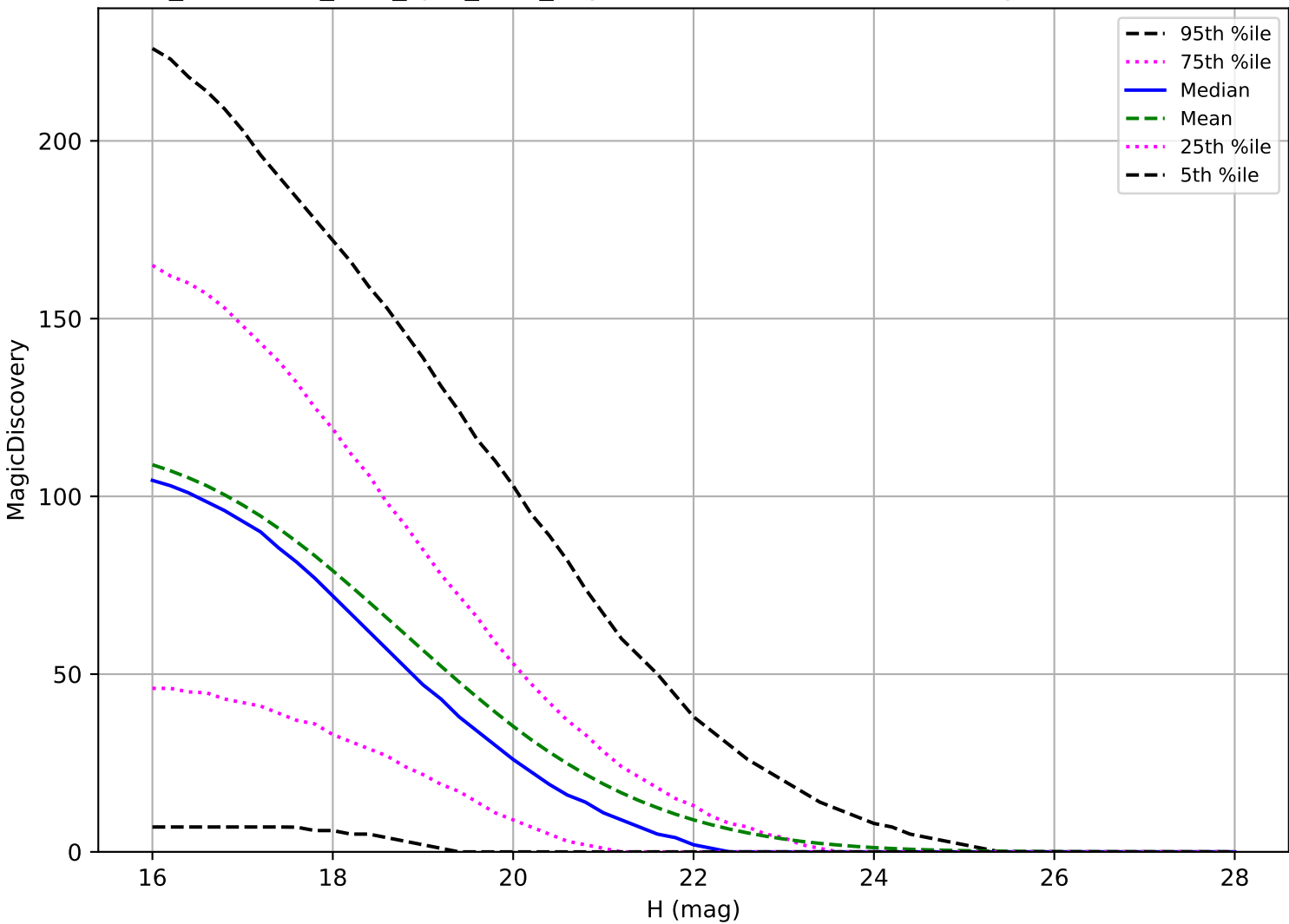
too_combined_s1.0_split_v3.4_10yrs: PHA 6 detections in 60 nights detection loss
