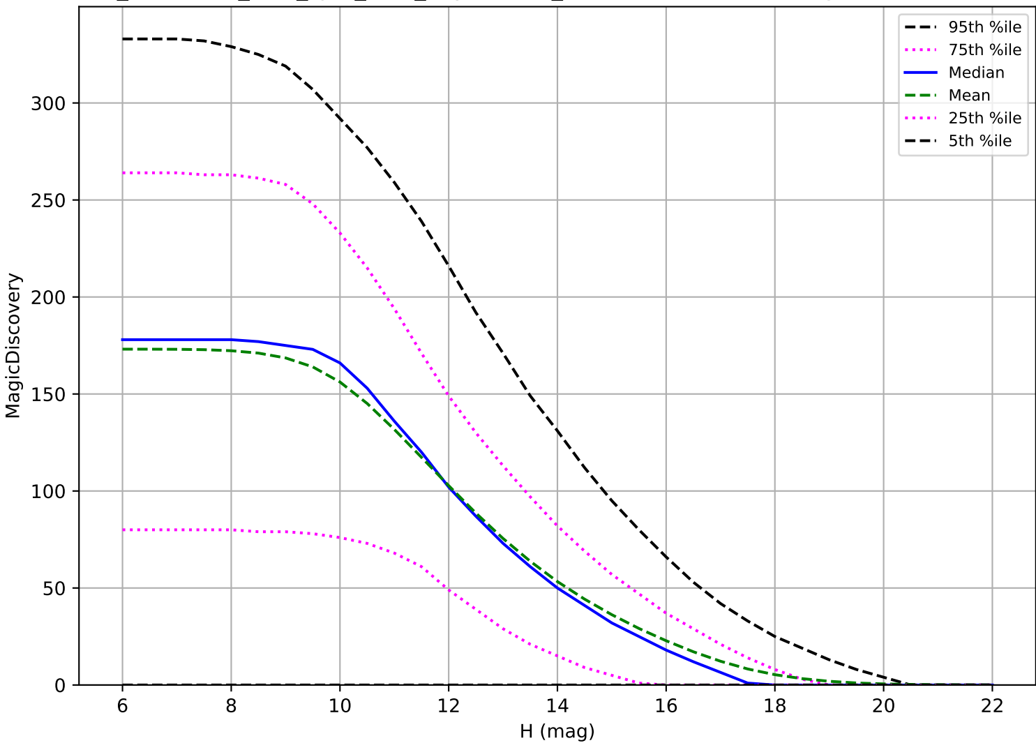
too_combined_s1.0_split_v3.4_10yrs: OCC_r5 6 detections in 60 nights detection loss
