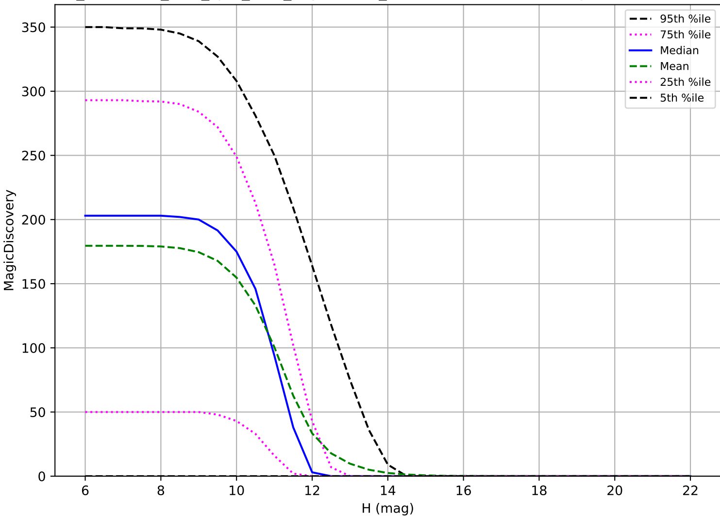
too_combined_s1.0_split_v3.4_10yrs: OCC_r20 6 detections in 60 nights detection loss
