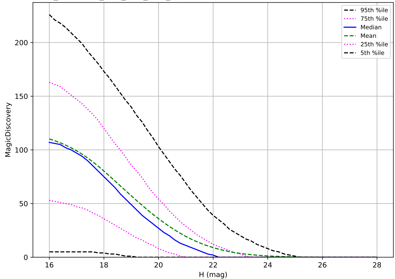
too_combined_s1.0_split_v3.4_10yrs: NEO 6 detections in 60 nights detection loss
