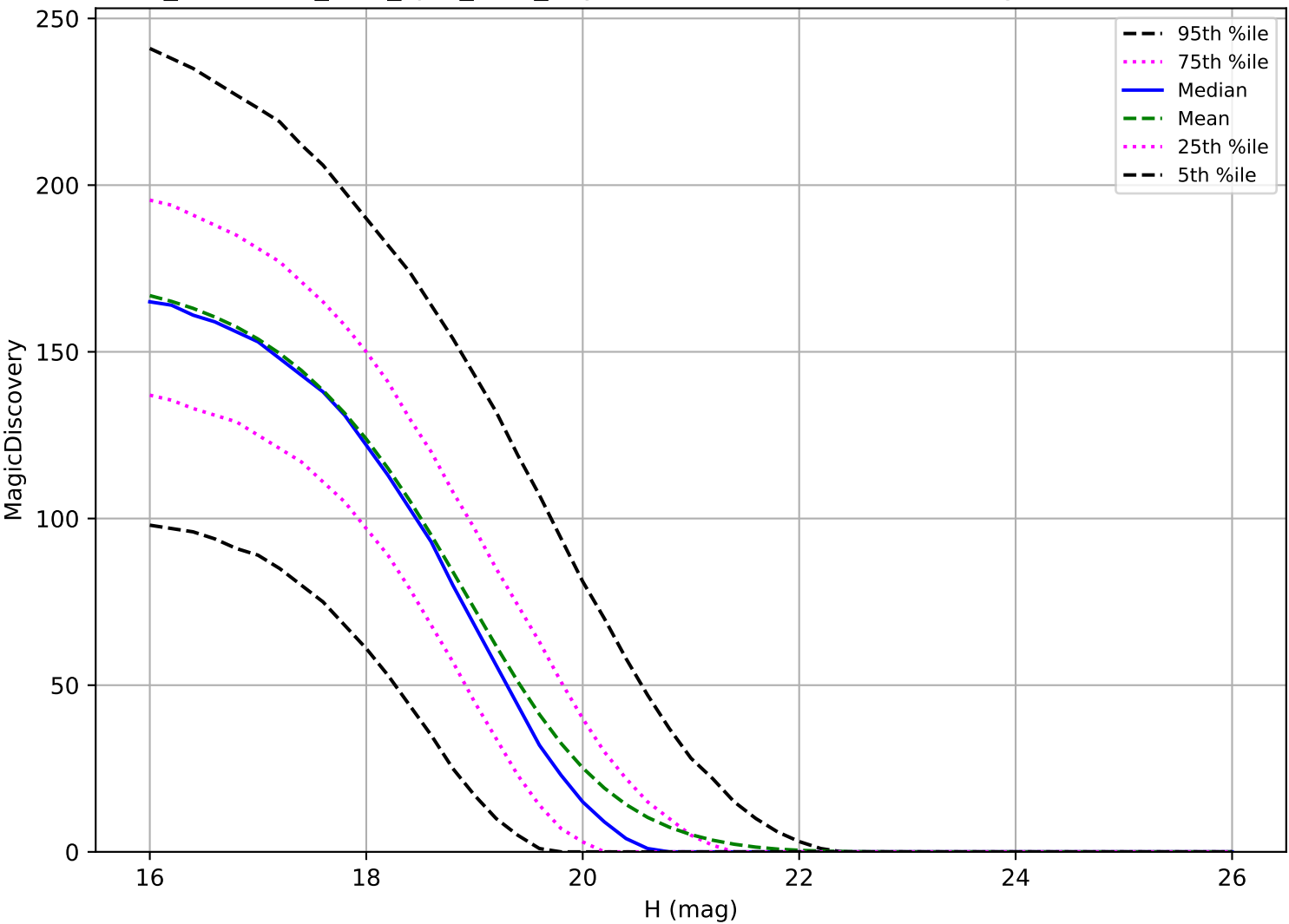
too_combined_s1.0_split_v3.4_10yrs: MBA 6 detections in 60 nights detection loss
