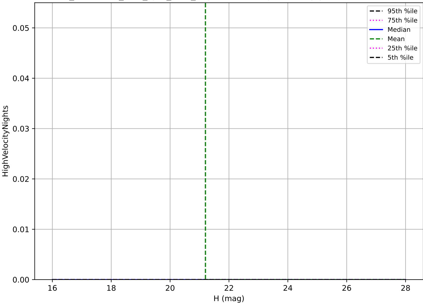
too_combined_s1.0_split_v3.4_10yrs: Vatira High velocity pair detection loss
