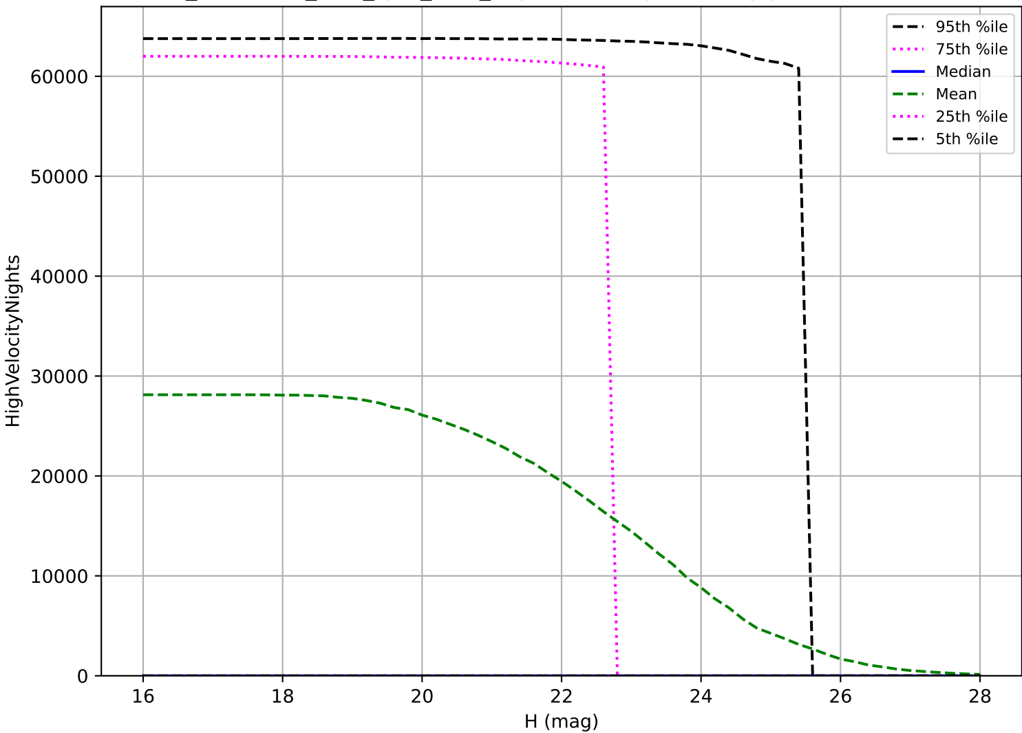
too_combined_s1.0_split_v3.4_10yrs: PHA High velocity pair detection loss
