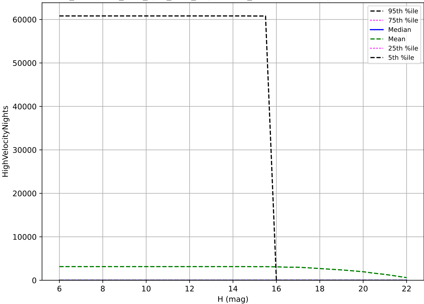
too_combined_s1.0_split_v3.4_10yrs: OCC_r5 High velocity pair detection loss
